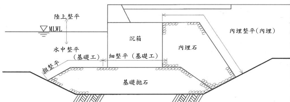
(2)重力式繫船碼頭(參考圖)
