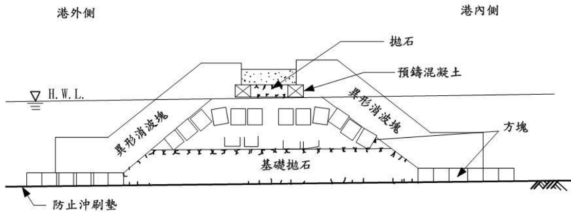
拋方塊式防波堤
